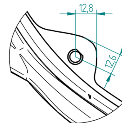
DETAIL J
