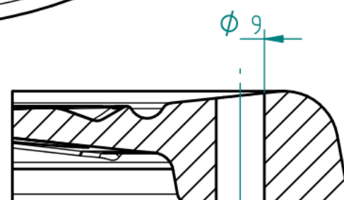
SECTION G-G
