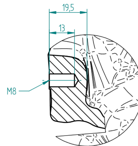
DETAIL K
