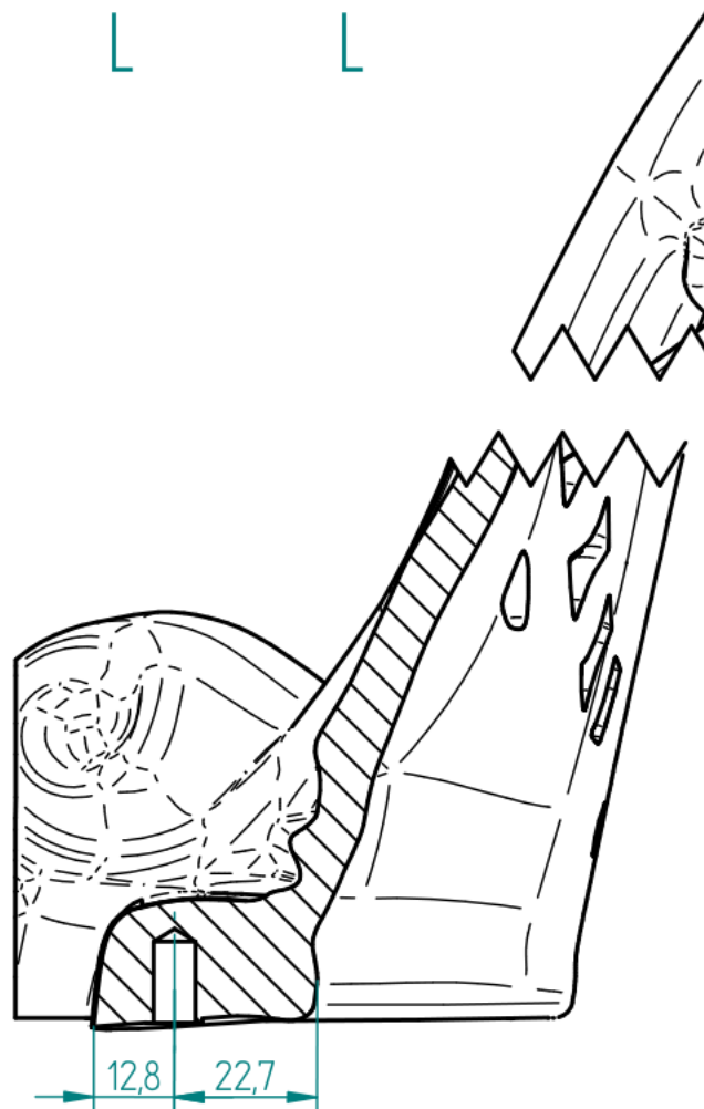
SECTION L-L
