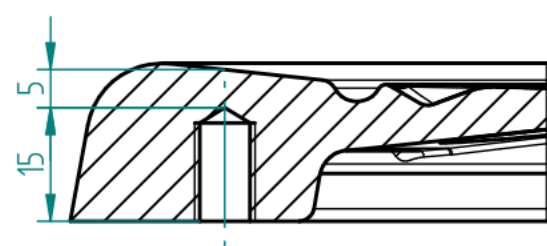
SECTION H-H
