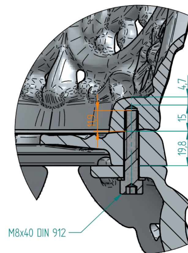
DETAIL D
